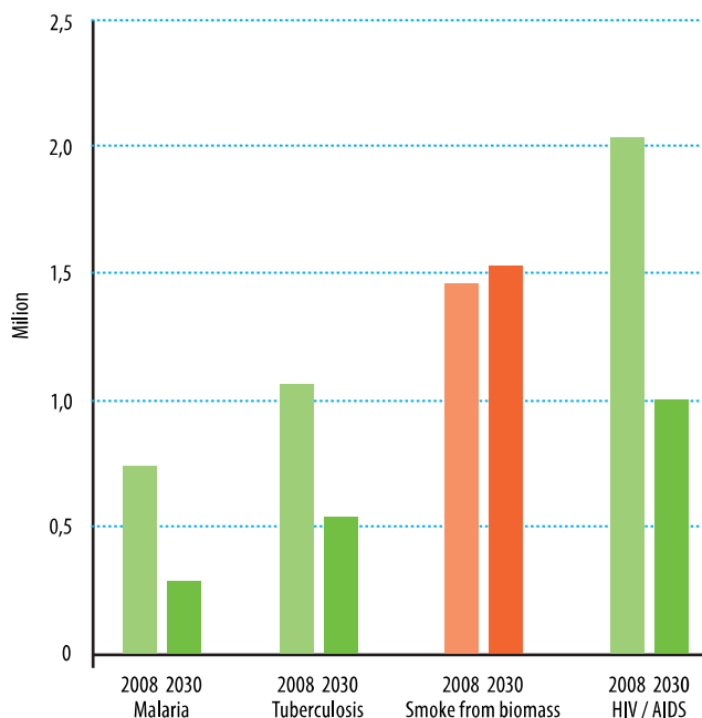
Figure 2: Premature annual deaths from household air pollution and other diseases
